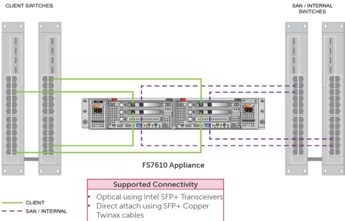
Figure 25 FS7610 network
