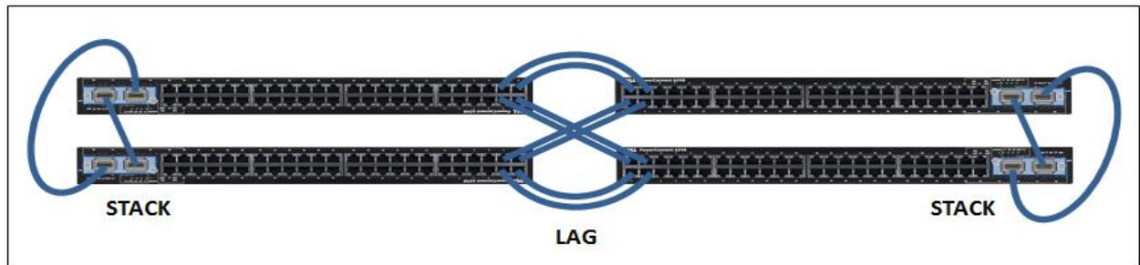
Figure 5 Using a LAG to interconnect switch stacks
