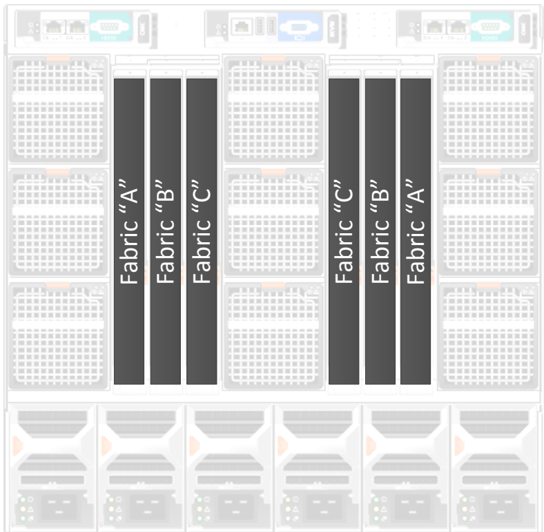
Figure 20 Blade I/O modules and M1000e Chassis
