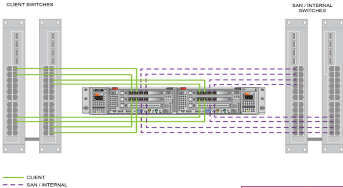
Figure 24 FS7600 network
