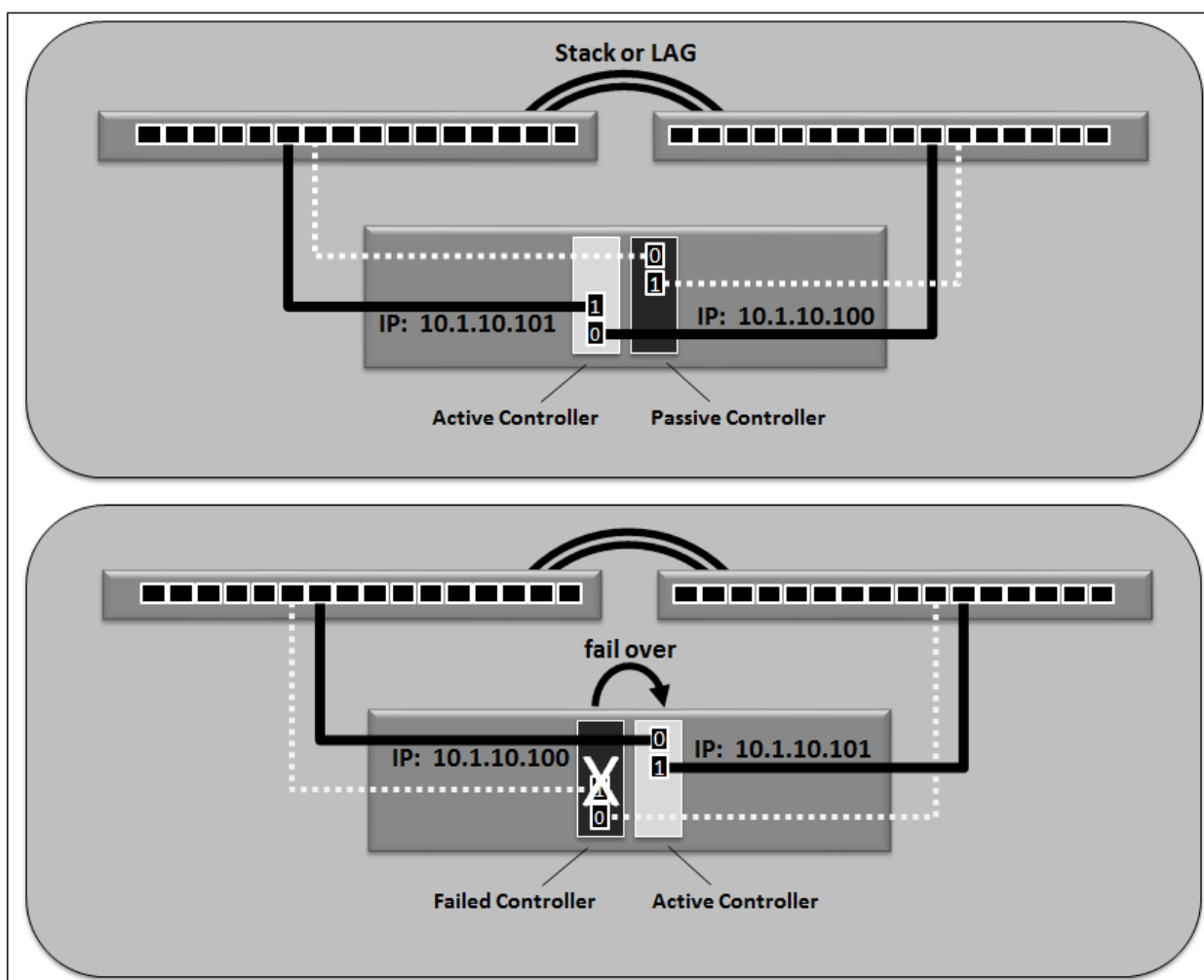
Figure 10 Fully connected controller failover
